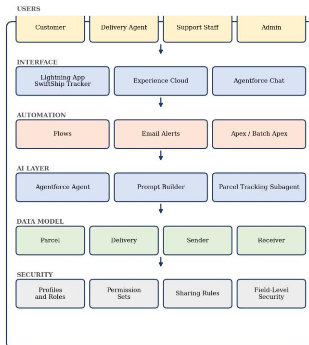
Figure 3: Solution architecture of SwiftShip Tracker
